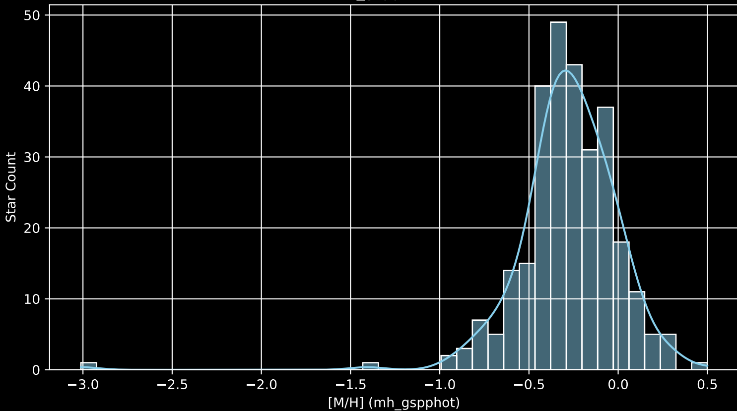
GALAH DR4 Field: [2397] [M/H] (mh_gspphot) (n= 288)
