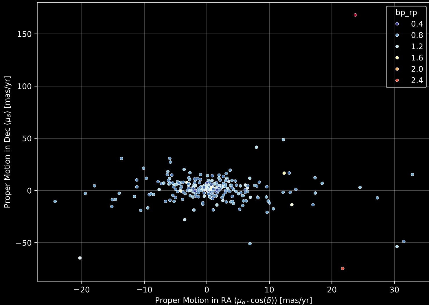
GALAH DR4 Field: [2397] Proper Motion Diagram (n= 289)
