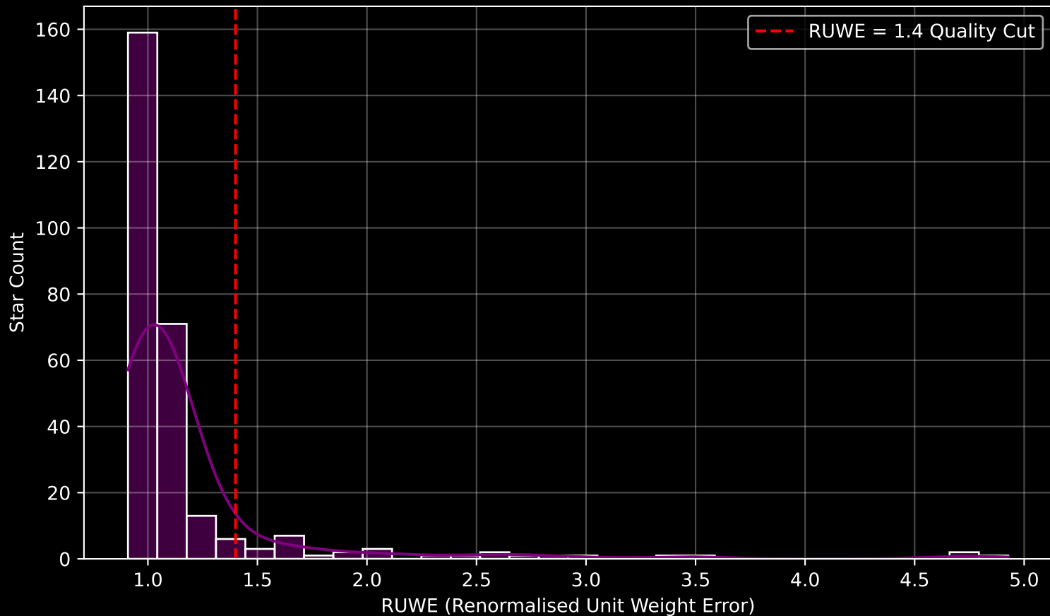
GALAH DR4 Field [2397] RUWE Distribution (n= 277)
