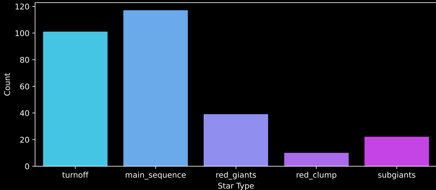
GALAH DR4 Field: [2397] Count plot of Star Type
